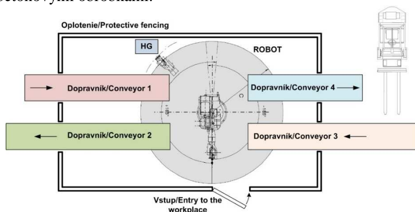
Obr. 1 Pôdorys pracoviska/ Ground plan of the workplace
