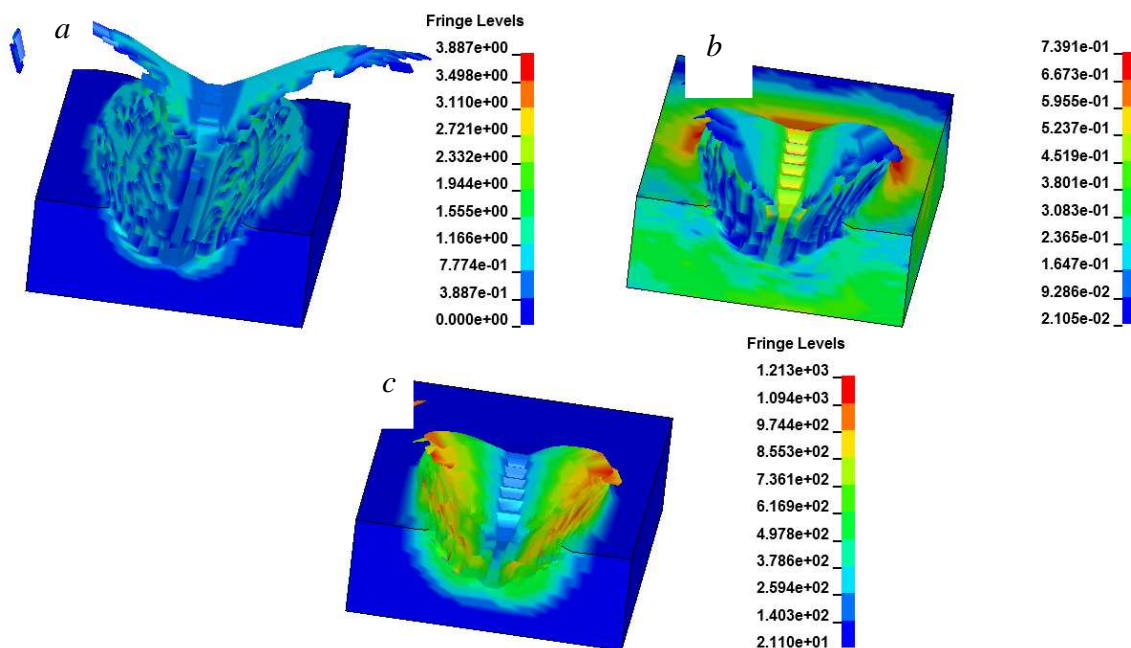
Fig. 1. Diagrams of the results for the workpiece in the processing by a single grain a - plastic deformation; b - shear strain; c - temperature
