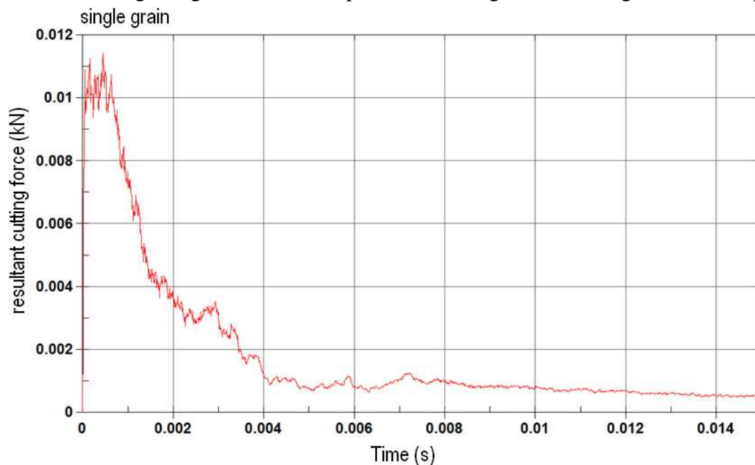
Fig. 2. The resultant cutting force by single grain
